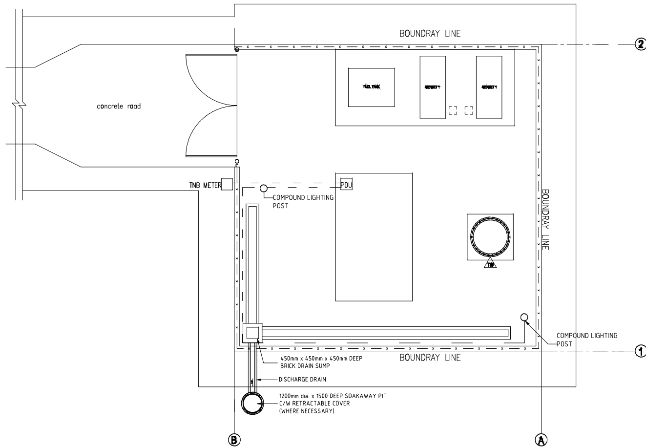
COMPOUND LAYOUT PLAN
