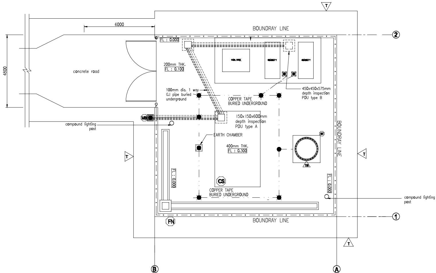
COMPOUND LAYOUT PLAN
