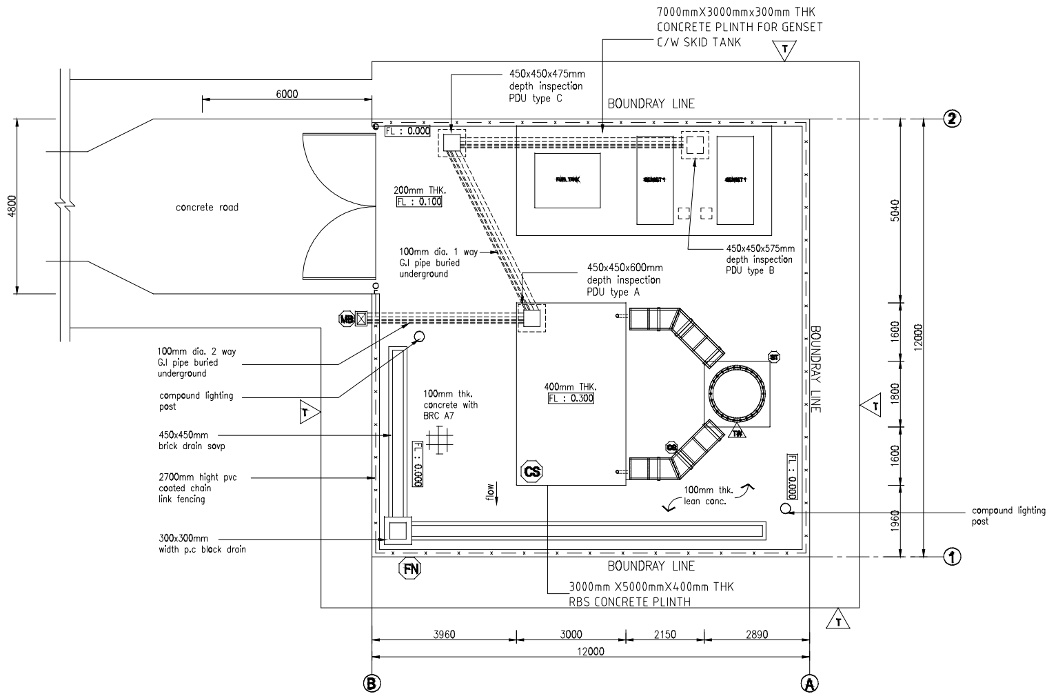
COMPOUND LAYOUT PLAN Scale = 1 : 100
