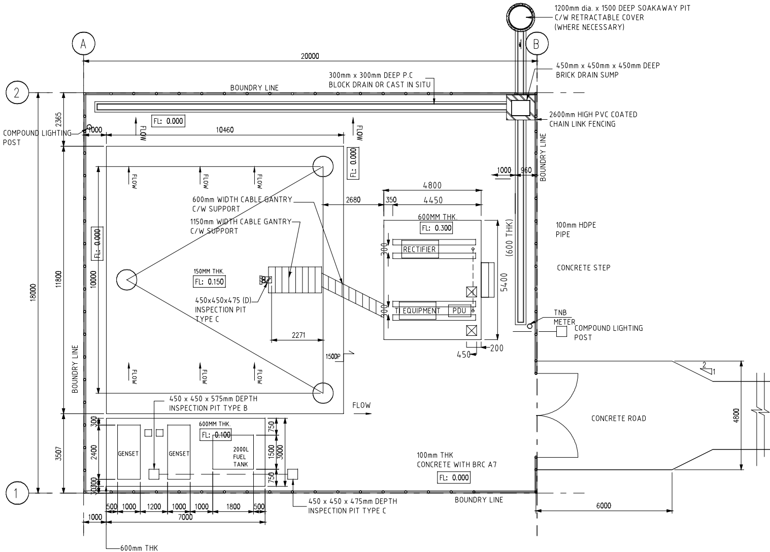
COMPOUND LAYOUT PLAN (20m x 18m)
